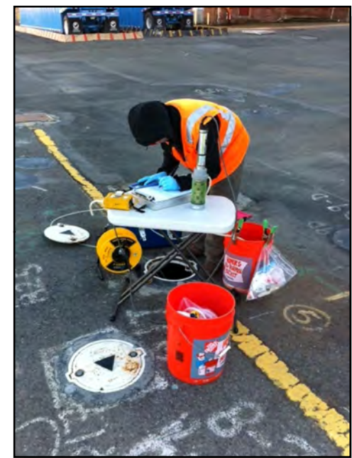
Groundwater Monitoring at IR15 Following Second Injection Event
