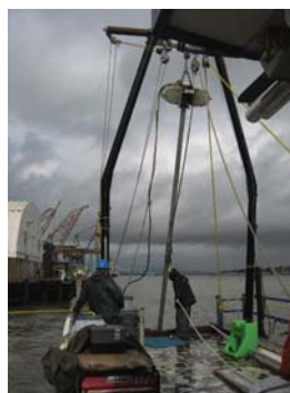
Positioning vibrocore barrel for a 30-foot sample at IA K
